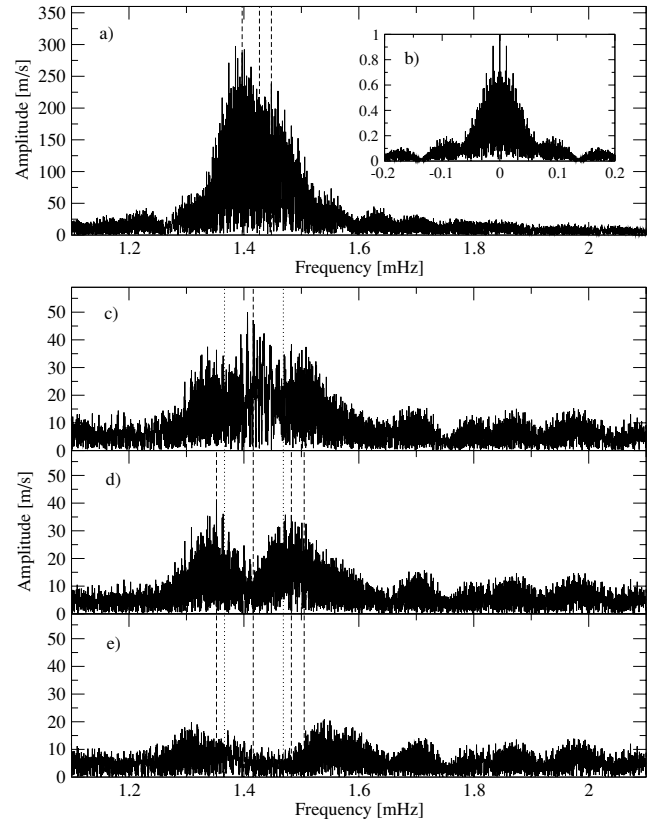
Figure 1. The amplitude spectra for the average Dy III RVs inferred from the UVES+SARG observations. (a) The DFT of the RV signal; (b) spectral window; (c) the residual amplitude spectrum obtained after pre-whitening the three main frequencies f_1\text{--}f_3 (dashed lines); (d) the residual amplitude spectrum obtained after pre-whitening the four frequencies f_1\text{--}f_4 ; (e) the residual noise after pre-whitening the seven frequencies f_1\text{--}f_7 from Table 3. These frequencies are indicated by dashed lines, while the dotted lines correspond to the MOST candidate frequencies.
