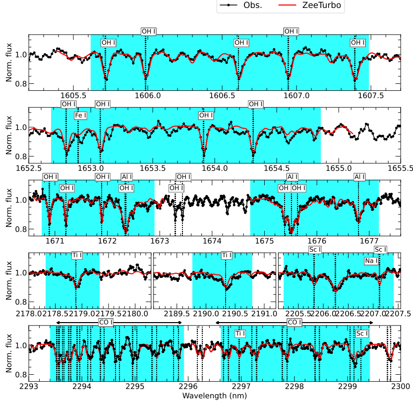
Fig. B.1. ZeeTurbo fitting process for the first observation of IRAS 04113+2758 N. The observed spectrum is shown in black, and the best fit model in red. Blue boxes indicate the regions used for parameter fitting, and the corresponding absorption lines are labelled.
