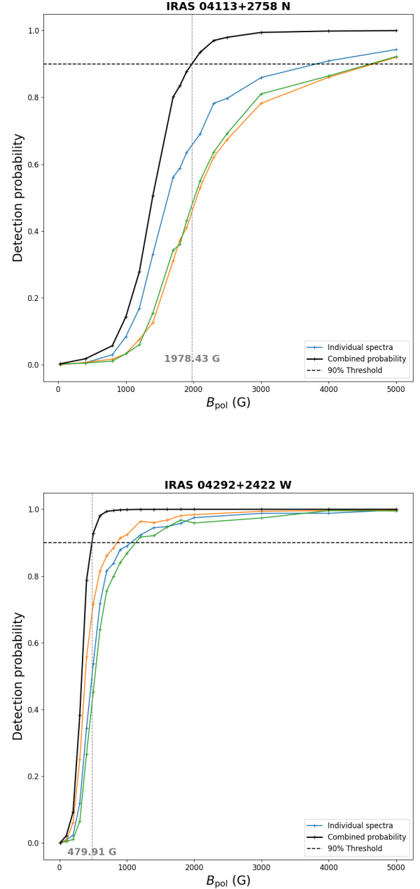
Fig. A.1. Example of dipolar magnetic detection probability curve as a function of the dipole strength. The colour curves represent the probability for each individual observation, while the black curve represents the combined probability for all observations. The 90 percent threshold is used to determine the field strength upper limit.
