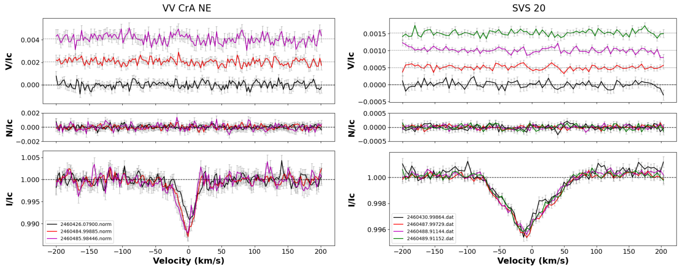
Fig. E.1. LSD profiles for each star. Different colours are used for the different observations. The Y-axes are I/I_c , N/I_c , and V/I_c , where I_c is the intensity of the stellar continuum. The I profile represents the total intensity, the Stokes V profile corresponds to the circular polarisation, and the Stokes N profile corresponds to the null spectra. Pixel size of 4.8 instead of 2.4 is applied for stars with v \sin i > 35 \text{ km s}^{-1} .
