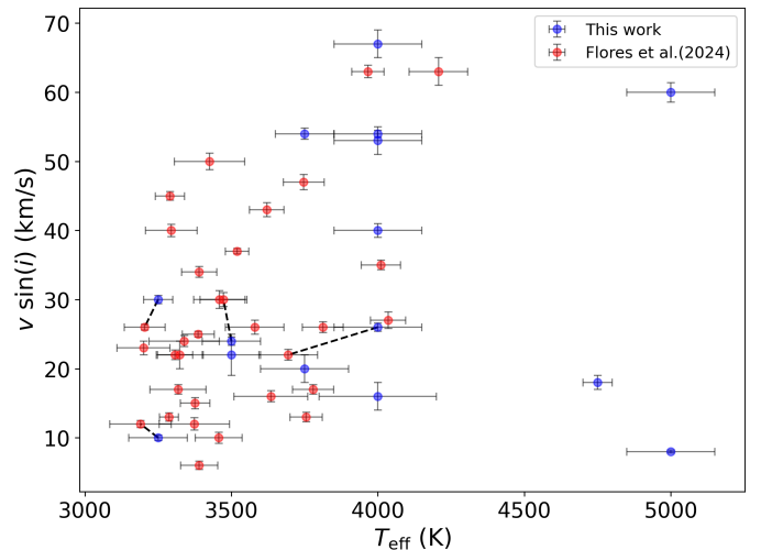
Fig. 5. Projected rotational velocities v \sin i , as a function of effective temperatures measured in this work (blue), and in the work of Flores et al. (2024) (red). The connected points with the dashed-line indicate the common stars in both samples.
