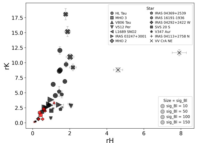
Fig. 4. Veiling in the K band as a function of the veiling in the H band for all observations of the sample. The size of the symbol is proportional to the uncertainty of the longitudinal magnetic field and each symbol corresponds to a different target. Magnetic stars are represented in red and stars without magnetic detections in black.
