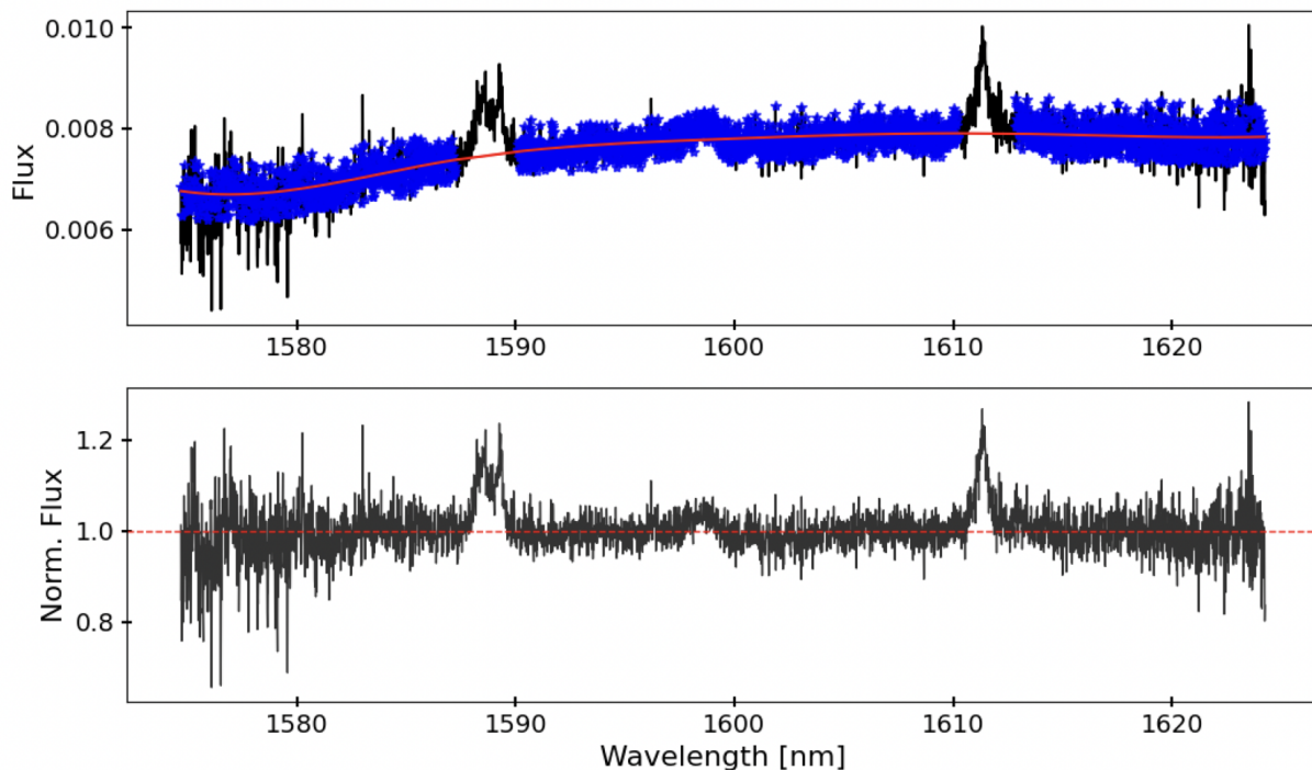
Fig. 1. Upper panel: order 32 of the spectrum of VV CrA SW without normalisation (black full line). In blue are the data points selected to fit the continuum using a sigma-clipping of 3 and 2 iterations. The spline fit of order 3 is plotted in red with a number of knots of 2. The two regions with emission lines were manually removed using the interactive tool. Lower panel: the same spectrum after normalisation. The dashed red line shows the continuum normalised to 1.
