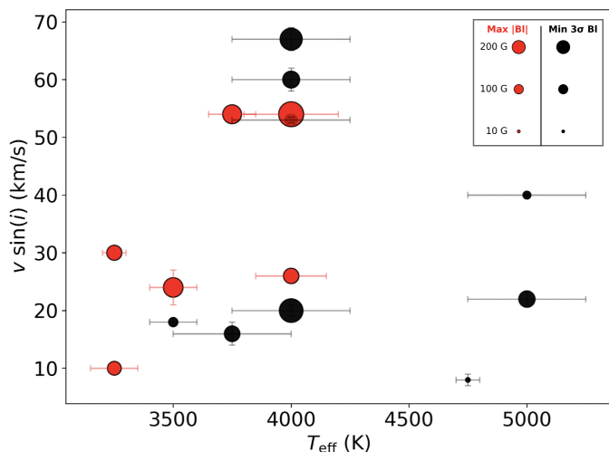
Fig. 3. The distribution of projected rotational velocity for each star of the sample as a function of effective temperature. Magnetic stars are represented in red and undetected magnetic stars in black. For the magnetic stars, the size of the symbols is proportional to the maximum absolute values of the longitudinal magnetic field. For the non-detected magnetic stars, it is proportional to the minimum of the 3\sigma uncertainty on B_\ell .
