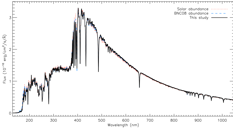
Fig. 7. Theoretical spectral energy distributions for the model atmosphere parameters T_{\text{eff}} = 7500 K, \log g = 4.1 and different chemical compositions of \alpha Cir. The LLMODELS flux spectra, convolved with a FWHM = 10 Å Gaussian profile, are presented for our final self-consistent model atmosphere with stratification included ( solid line ), chemically-homogeneous solar abundance model ( dotted line ), and a model computed for BNC08 abundances ( dashed line ).
