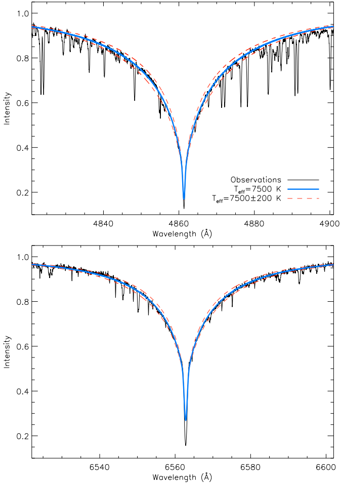
Fig. 9. Comparison of the observed and theoretical H \alpha and H \beta line profiles of \alpha Cir. Observations are shown by the thin line. Thick solid line gives the hydrogen line profiles computed for our final self-consistent, chemically-stratified model atmosphere with T_{\text{eff}} = 7500 K, \log g = 4.1 . Dashed lines show the effect of changing T_{\text{eff}} by \pm 200 K.
