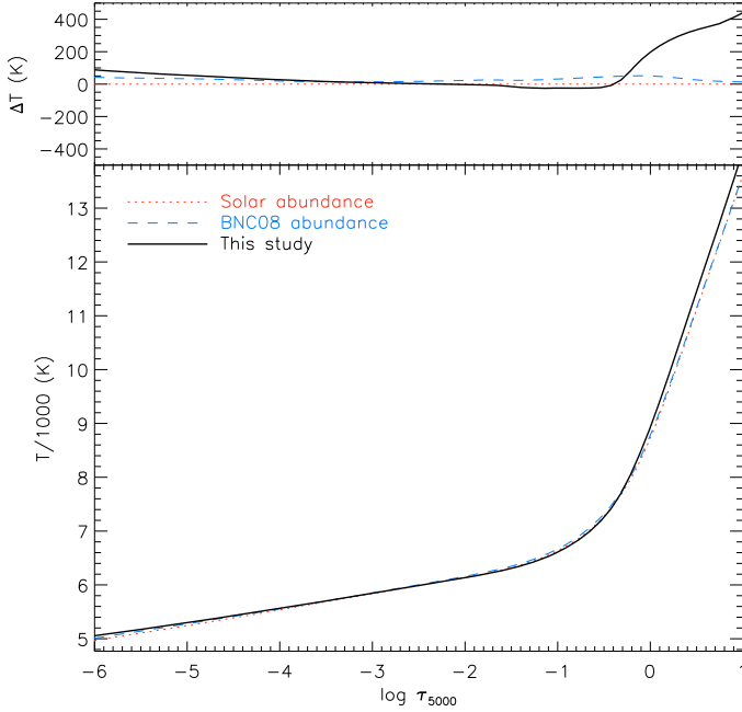
Fig. 11. Temperature as a function of standard optical depth, \tau_{5000} , for the final self-consistent model atmosphere of \alpha Cir with T_{\text{eff}} = 7500 K, \log g = 4.1 (solid line) compared to the temperature structure of the models with the same atmospheric parameters but using homogeneous solar (dotted line) and BNC08 (dashed line) abundances. The upper panel shows the temperature differences with respect to the solar-abundance case.
