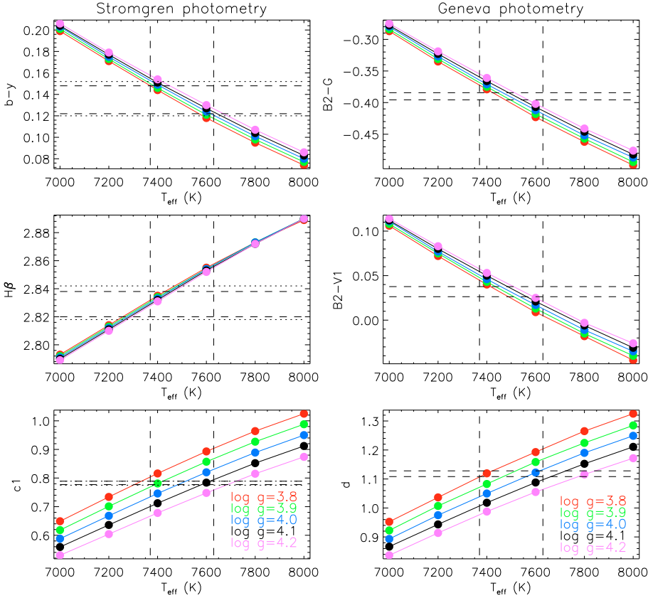
Fig. 8. Dependence of the synthetic Strömgen (left panel) and Geneva (right panel) photometric parameters on the T_{\text{eff}} and \log g for the models with stratified chemical composition. The theoretical temperature ( b - y , H\beta for the Strömgen and B2 - G , B2 - V1 for the Geneva photometry) and gravity ( c_1 for the Strömgen and d for the Geneva photometry) indicators are compared with the corresponding observed parameters. Those are indicated by the horizontal dashed lines showing \pm 1\sigma ranges and by the dotted lines (Strömgen photometry only) showing the minimum and maximum observed values. The vertical dashed lines correspond to the 7500 \pm 130 K T_{\text{eff}} range.
