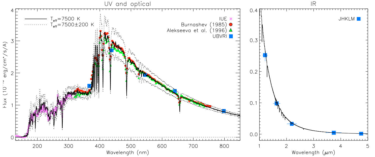
Fig. 6. Comparison between the observed ( symbols ) and theoretical ( lines ) spectral energy distribution of \alpha Cir. Photometric and spectrophotometric observations, covering the wavelength range from the ultraviolet and optical ( left panel ) to the infrared ( right panel ), are discussed in the text (see Sect. 2). The solid line shows the theoretical energy distribution computed for the final self-consistent model atmosphere of \alpha Cir with parameters T_{\text{eff}} = 7500 K and \log g = 4.1 . The dotted lines illustrate the effect of changing T_{\text{eff}} by \pm 200 K. The LLMODELS flux spectra are convolved with a FWHM = 10 Å Gaussian profile.
