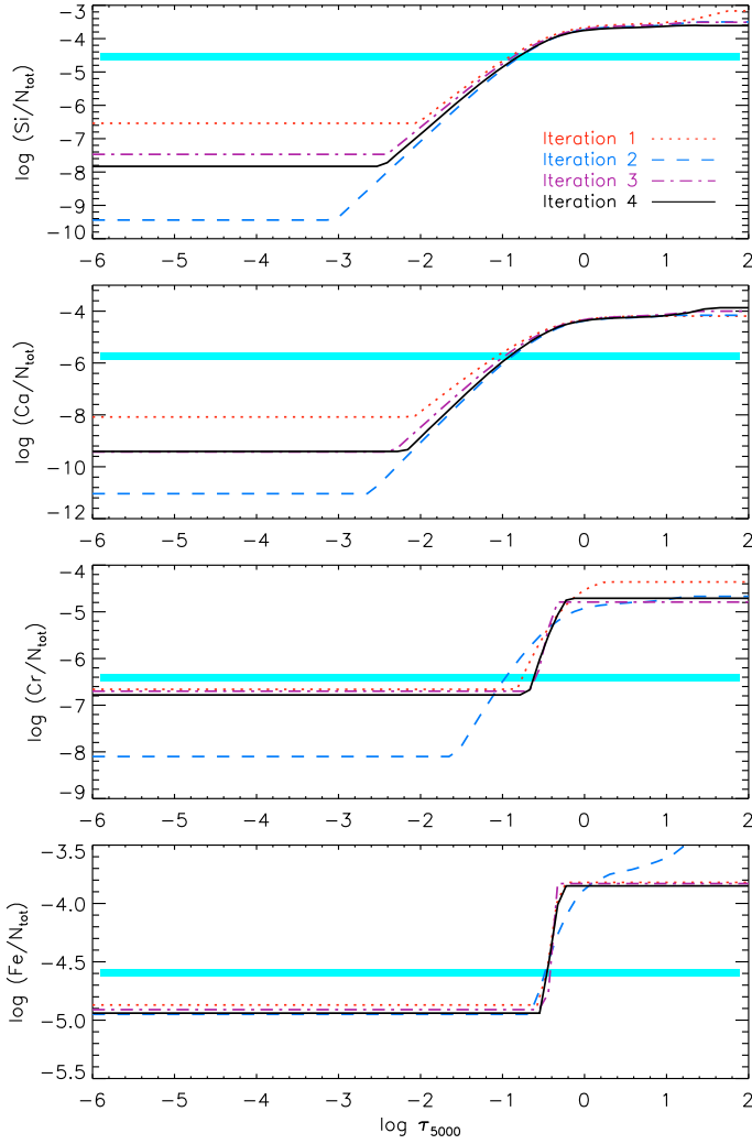
Fig. 5. Vertical distribution of Si, Ca, Cr, and Fe abundance in the atmosphere of \alpha Cir for different iterations of the stratification analysis. The thick solid line corresponds to the final element distribution. The light horizontal bar shows solar abundances.
