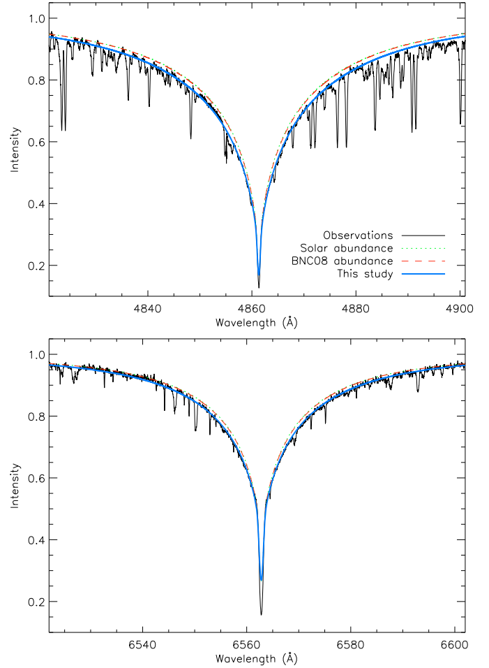
Fig. 10. Comparison of the observed and theoretical H \alpha and H \beta line profiles of \alpha Cir. Observations are shown by the thin solid line. Theoretical calculations with parameters T_{\text{eff}} = 7500 K, \log g = 4.1 are presented for our final self-consistent model atmosphere with stratification included (thick solid line), chemically-homogeneous solar abundance model (dotted line), and a model computed for BNC08 abundances (dashed line).
