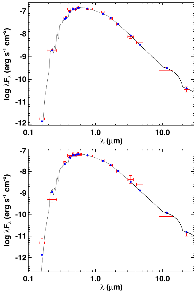
Figure 2. SEDs for \rho CrB (top) and 88 Leo (bottom). Red symbols are the observed photometric measurements, where the horizontal bars represent the effective width of the passband. Blue symbols are the model fluxes from the best-fit Kurucz atmosphere model (black).
