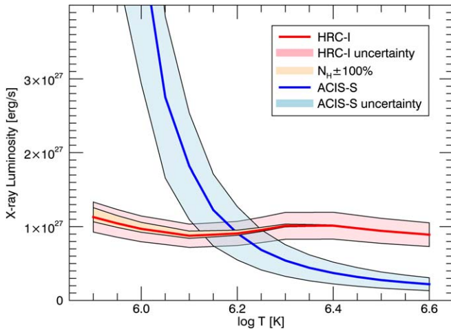
Figure 3. The X-ray luminosity of \rho CrB for isothermal, collision-dominated, optically thin plasma radiative loss as a function of plasma temperature implied by the observed Chandra HRC-I and ACIS-S count rates. Shaded regions indicate the uncertainties arising from the count rate measurements and a 100% error in the assessment of the intervening neutral hydrogen column density.
