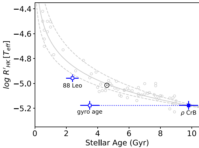
Figure 5. Chromospheric activity vs. stellar age for a sample of spectroscopic solar twins from Lorenzo-Oliveira et al. (2018) with ages determined from isochrone fitting (gray circles). The asteroseismic age of \rho CrB is overplotted as a filled square, while updated ages from gyrochronology for both stars are shown with open squares.
