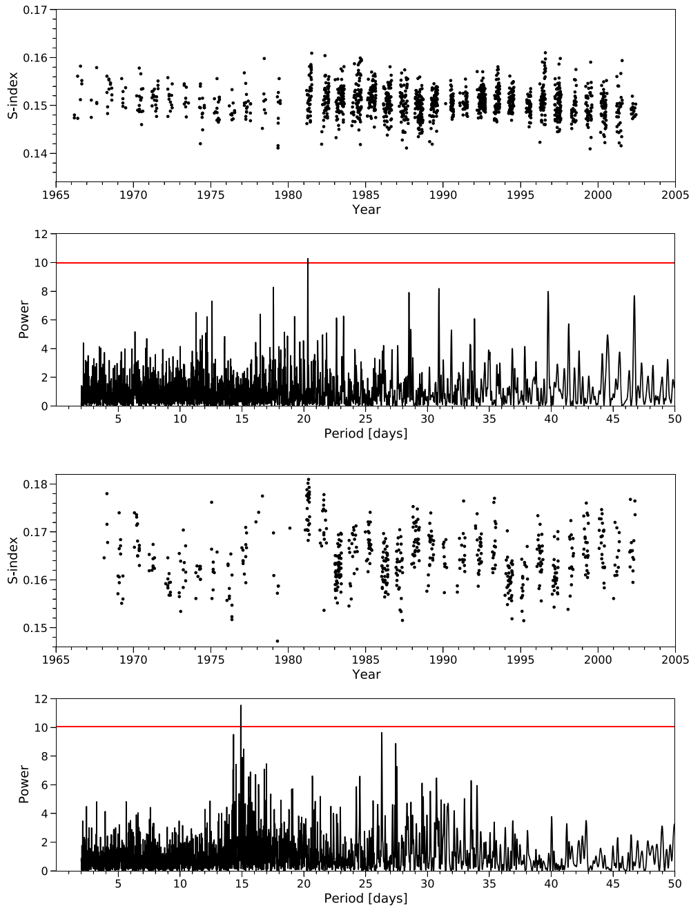
Figure 1. Time series and Lomb–Scargle periodograms for \rho CrB (top two panels) and 88 Leo (bottom two panels) showing the recovered rotation signals of 20.3 and 15.0 days, respectively. Red lines in the periodograms indicate the 5% FAP calculated from a Monte Carlo process.
