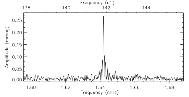
Figure 14. The pulsation mode in TIC 49818005.
