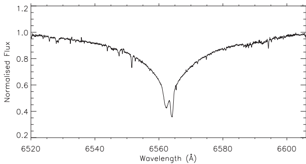
Figure A14. The SALT/HRS spectrum of the H_{\alpha} line in TIC 410163387 showing the star to be a spectroscopic binary system.
