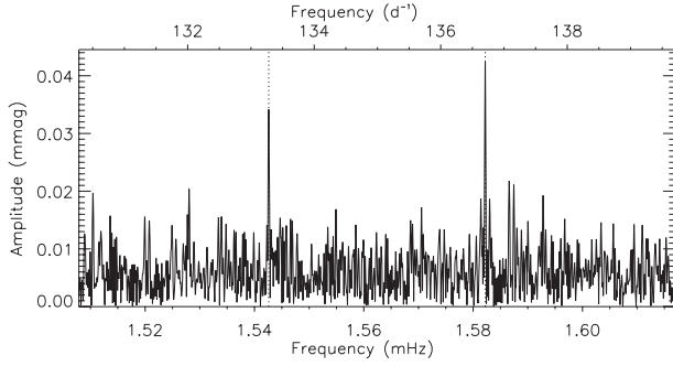
Figure 26. The pulsation signatures seen in TIC 146715928. The vertical dotted lines represent the extracted peaks, which are separated by 40 \mu Hz.
