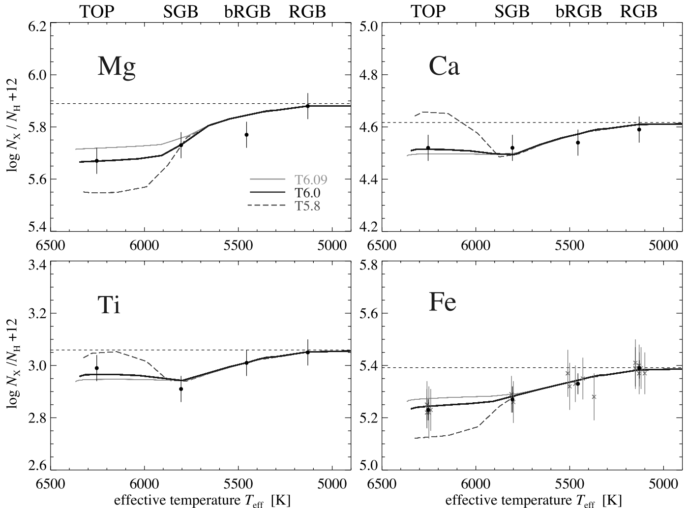
FIG. 6.—Observed trends of elemental abundances with evolutionary stage ( filled circles with error bars ) compared to predictions from stellar evolution models including atomic diffusion and turbulent mixing with three different efficiencies. Note how the T5.8 model falls below or above the best-fitting T6.0 model depending on the element (likewise the T6.09 model). For details, see text. [See the electronic edition of the Journal for a color version of this figure.]
