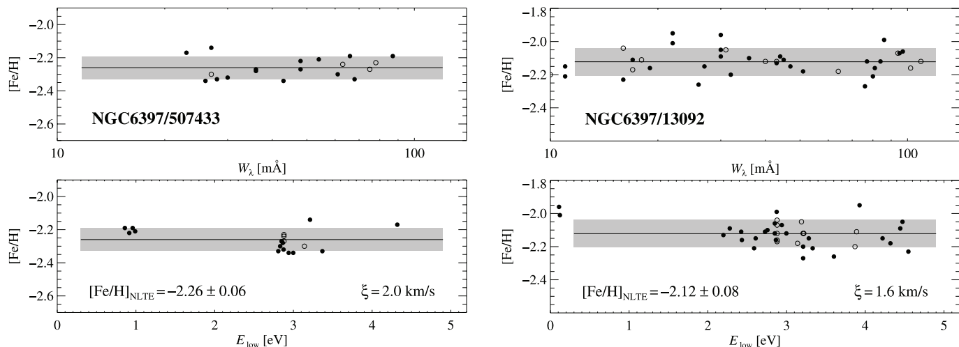
FIG. 5.— Individual line abundances of Fe I ( filled circles ) and Fe II ( open circles ) lines as a function of line strength ( top ) and excitation energy of the lower level E_{low} ( bottom ) for a TOP star and an RGB star, respectively. While there is no obvious trend of [Fe/H] with E_{low} , this is not true for all targets and we do not use the excitation equilibrium as an additional effective temperature indicator.
