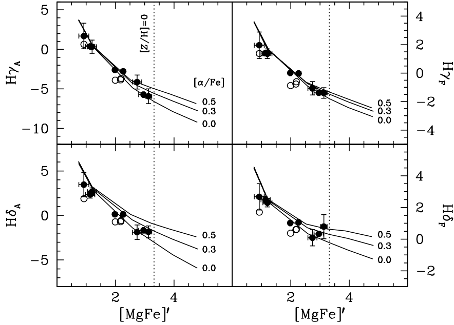
Figure 1. The \alpha/\text{Fe} -independent index [\text{MgFe}]' versus H\gamma_A , H\gamma_F , H\delta_A and H\delta_F as functions of total metallicity, for the abundance ratios [\alpha/\text{Fe}] = 0.0, 0.3, 0.5 (see labels), and a fixed age of 12 Gyr. The vertical dotted line indicates the [\text{MgFe}]' of the solar metallicity model. Circles are the indices measured on the integrated light of galactic globular clusters (Puzia et al. 2002). Open circles are globular clusters with horizontal branches that are relatively red given their metallicity (see Maraston et al. 2003).
