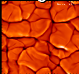
red giant
