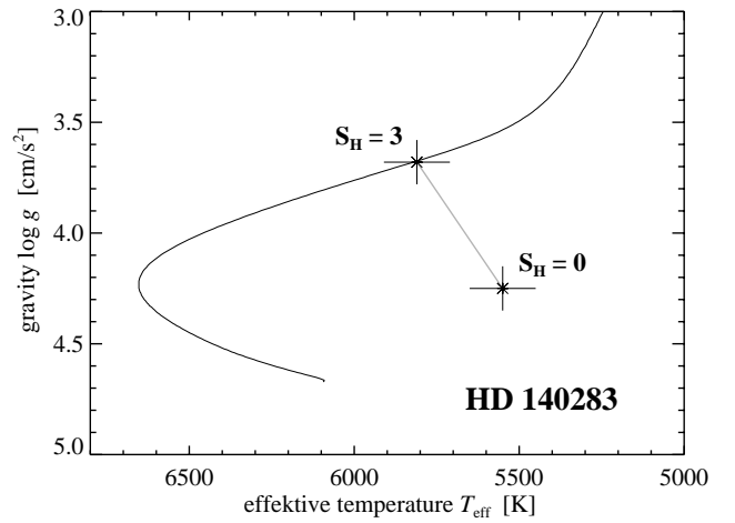
Fig. 2. A comparison between the stellar parameters of HD 140283 for different assumptions concerning the efficiency of hydrogen collisions. S_{\text{H}} = 3 corresponds to our best estimate and places this star in a subgiant phase of evolution. A mass close to 0.8 M_{\odot} is indicated from a track of appropriate metallicity by VandenBerg et al. (2000). However, assuming S_{\text{H}} = 0 (no collisions) results in a T_{\text{eff}}\text{-log } g combination in irreconcilable conflict with the star's known properties, both in terms of its evolutionary stage and mass.
