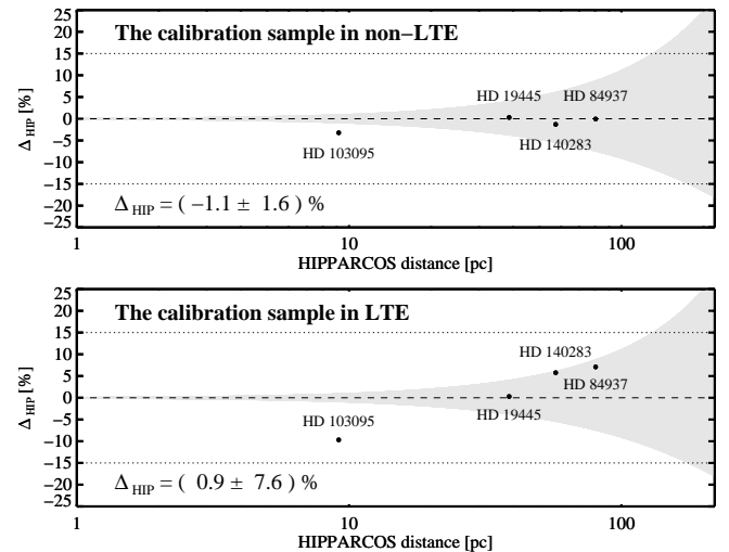
Fig. 4. \Delta_{\text{HIP}} as a function of the astrometric distance, both in non-LTE (top) and LTE (bottom). The grey wedge indicates the typical uncertainty of the HIPPARCOS parallaxes. When non-LTE gravities are considered the star-to-star scatter is significantly reduced.
