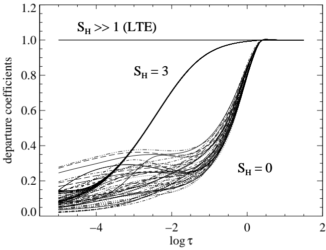
Fig. 1. Departure coefficients b_i for Fe I terms in HD 140283 as a function of the optical depth \log \tau_{5000} . It becomes evident that they depend drastically on S_{\text{H}} . The line source functions are Planckian for all models with S_{\text{H}} > 0 , but not for the S_{\text{H}} = 0 model. The best model ( S_{\text{H}} = 3 ) already returns abundances quite close to LTE.
