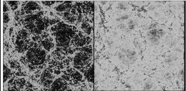
Cold dark matter
