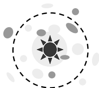
Feedback from star formation kicks in. Young, hot stars ionize part of the gas. Stellar winds and supernovae blow the gas outwards – some of it may leave the halo
