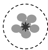
Stars form in the cooled gas
