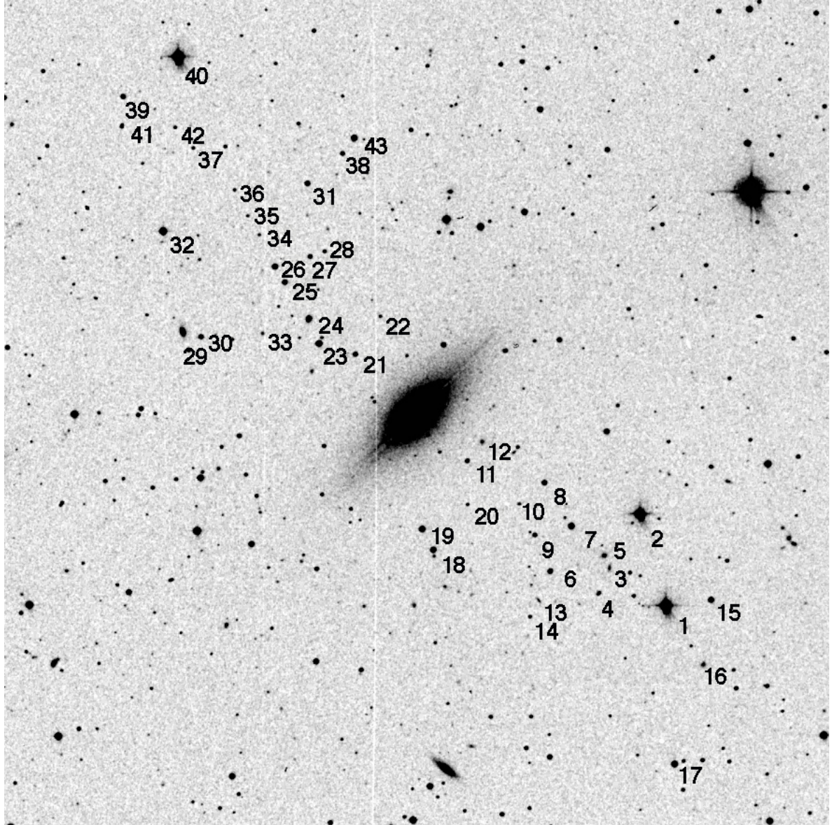
Figure 1: 25' \times 25' optical image of the edge-on active galaxy ESO 666-01 (centre). Numbers refers to objects for which data is given in Table 1. The label is typically located to the lower right of each object. The white vertical lines (most notably right across the disk of ESO 666-01) in this image are caused by bad columns on the telescope CCD.
