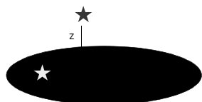
Galactic coordinates
