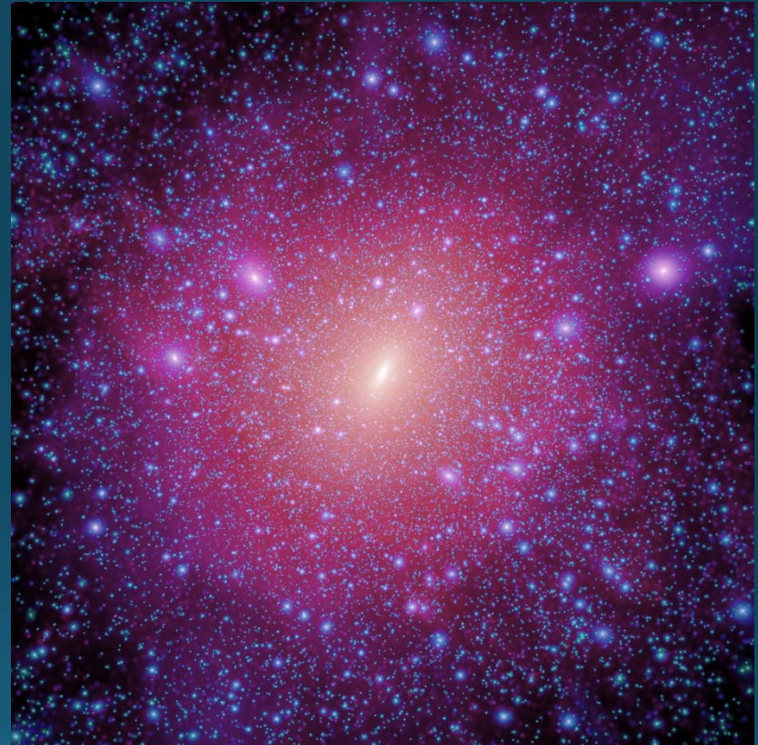
Dark matter halo from the Aquarius simulation
