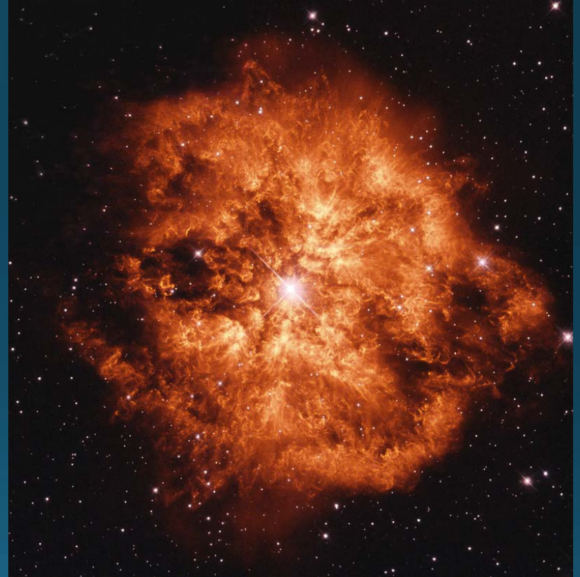
A Wolf-Rayet star (high-mass star with huge ionizing flux and mass loss due to winds)
