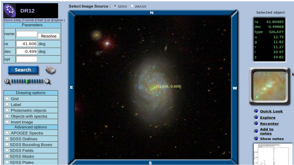
Fig.3. Center the green square at the object of interest. Try not to center it on a foreground star. The box in the upper, right corner shows the coordinates (right ascension, declination) in degrees. It also shows the galaxy type and the apparent magnitudes of the object in five different bands. In the lower right corner, is “Explore” that takes you to the page with additional information about the object and its optical spectrum.
