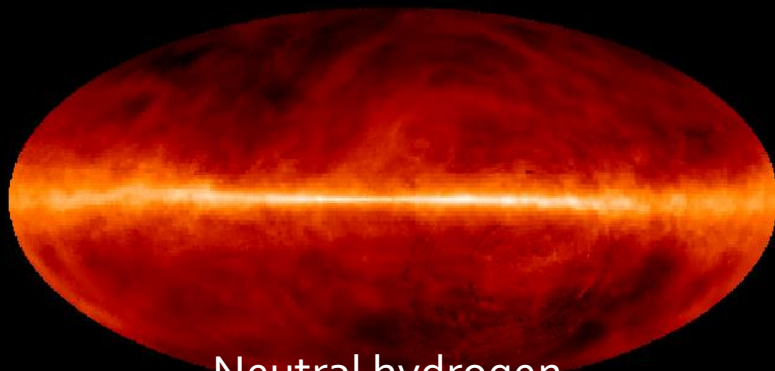
Neutral hydrogen
