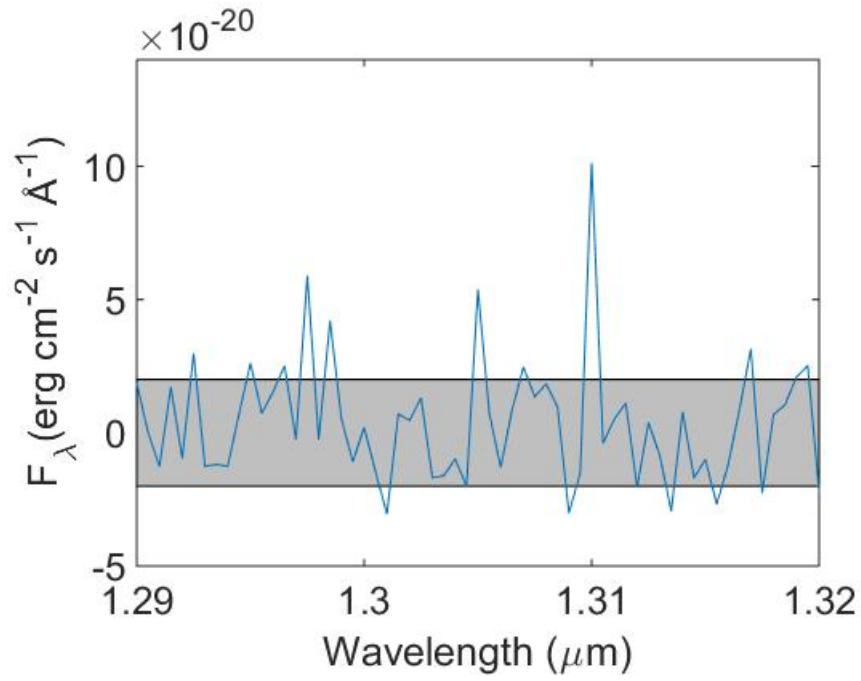
Figure 2: The near-infrared spectrum (at 5 Å resolution) of the high-redshift galaxy candidate. The 1\sigma uncertainty on the flux is indicated by the gray region. The data supposedly shows an emission feature at \lambda \approx 1.31 \mu\text{m} (13100 Å), detected at the \approx 4\text{--}5\sigma level.
