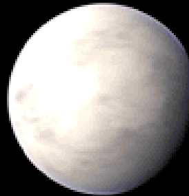
#3 Kepler-22 b
