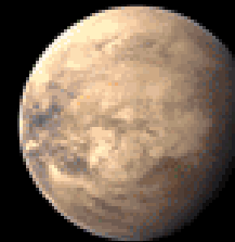
#4 HD 85512 b
