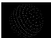
Dyson-bubbla
