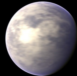
Kepler-22 b
