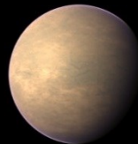
Kepler-62 f
