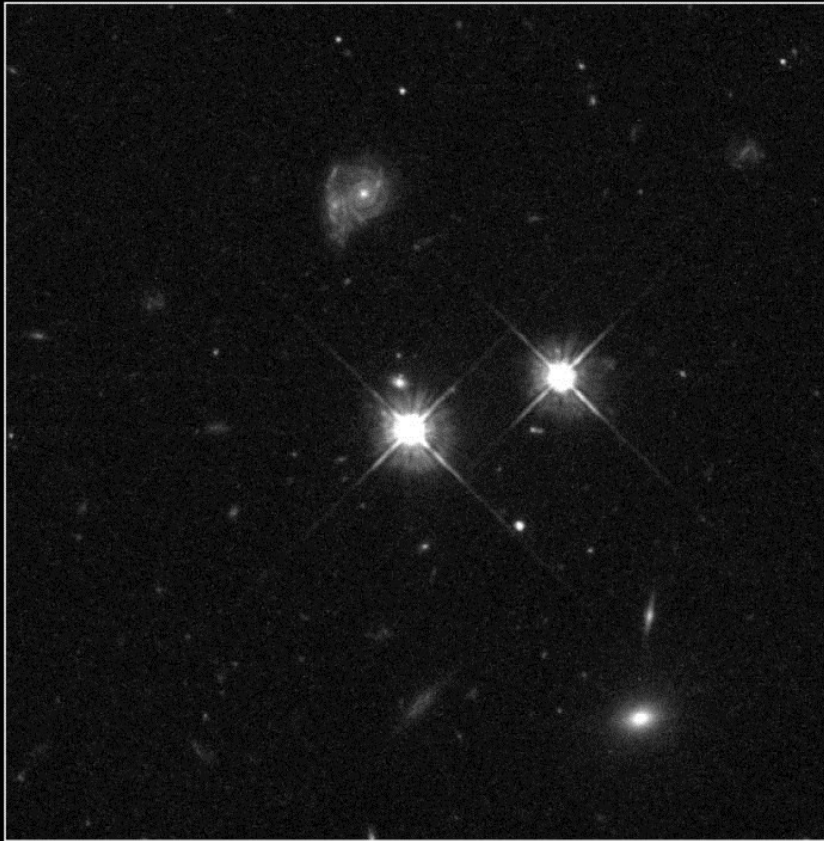
HST's 100,000th Observation
