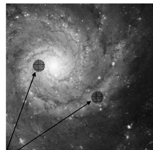
Dyson-signaturer
