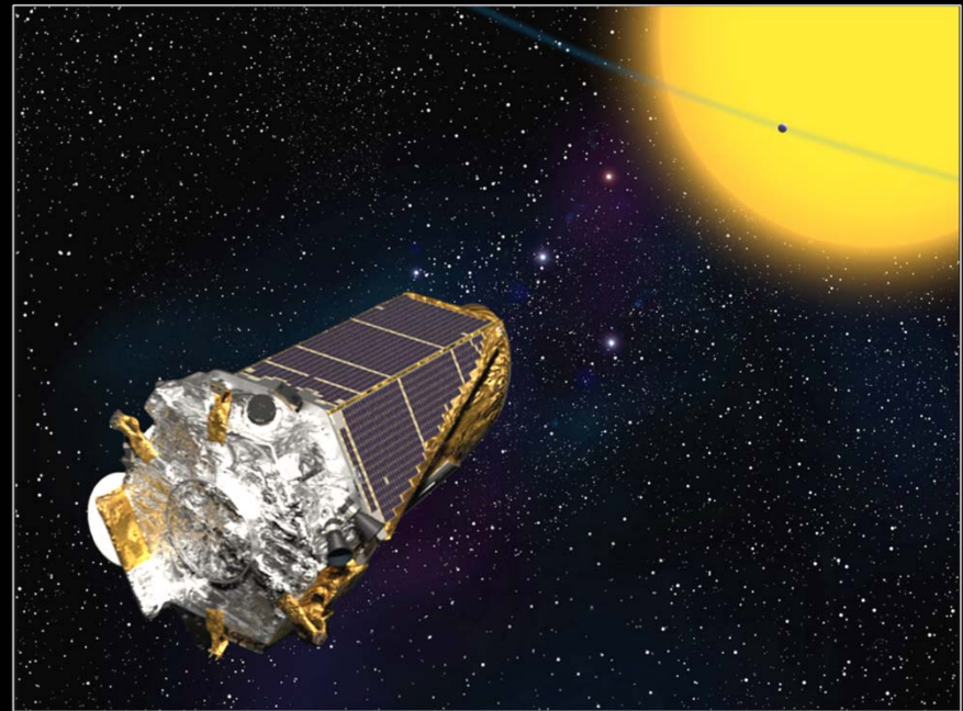
Kepler-satelliten
