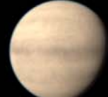
[38 ly] GJ 180 c*
