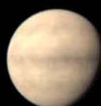
[49 ly] GJ 163 c
