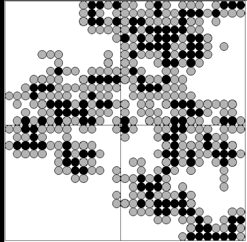
Perkolationsimulering
