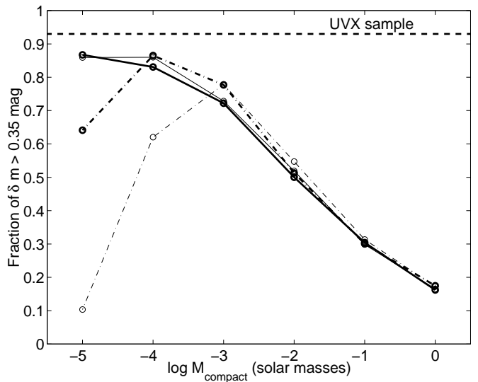
Fig. 5. The fraction of objects with amplitudes higher than 0.35 magnitudes predicted by microlensing scenarios for different M_{\text{compact}} , assuming \Omega_{\text{compact}} = 0.3 , \sigma_{v,\text{compact}} = 600 km/s and R_{\text{QSO}} = 10^{12} m (thick solid), 3 \times 10^{12} m (thin solid), 10^{13} m (thick dash-dotted), 3 \times 10^{13} m (thin dash-dotted). The thick dashed line marks the observed fraction (93%) of the UVX quasar sample.
