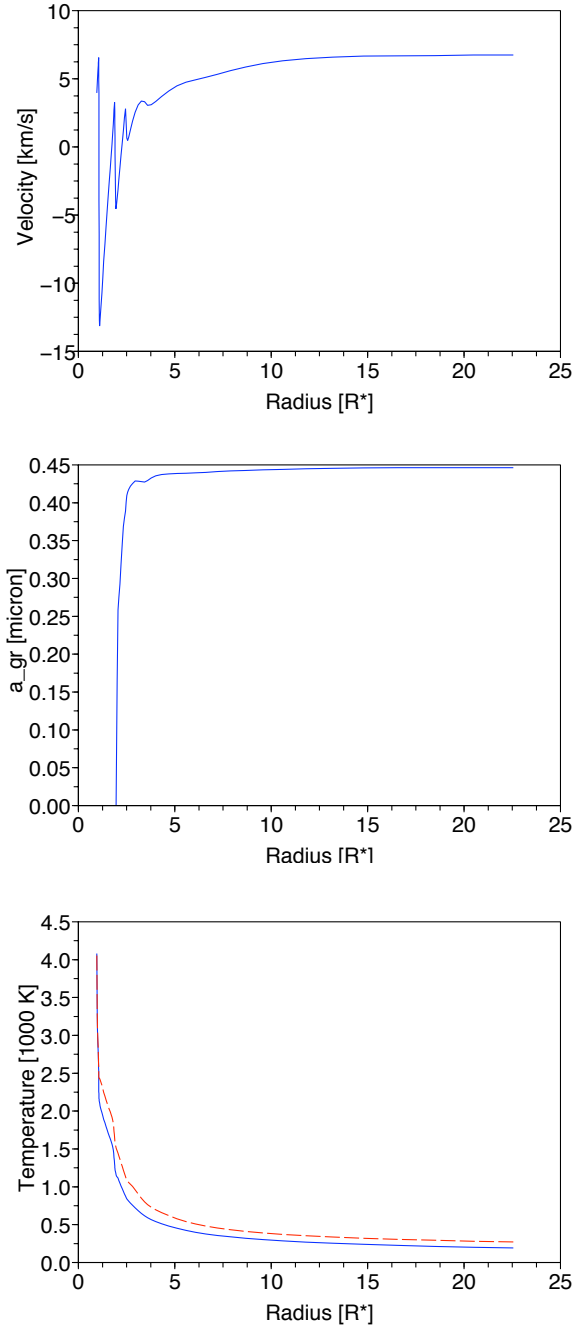
Fig. 2. Snapshot of the spatial structure of model B with n_{\text{gr}}/n_{\text{H}} = 1 \cdot 10^{-15} : top: velocity, middle: grain radius, bottom: grain temperature (solid) and gas temperature (dashed).
