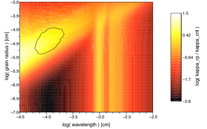
Fig. 1. Opacity \kappa_{\text{rp}} of forsterite grains in units of the critical opacity \kappa_{\text{crit}} ( M_* = 1M_\odot , L_* = 7000L_\odot ), assuming that 30 percent of Si is condensed into grains; The black contour shows the region where the flux-weighted opacity exceeds the critical opacity, assuming a Planckian flux distribution with T_* = 2700 K.
