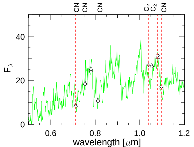
Fig. 10. Comparison of a l52t30c20u2pm20 minimum model spectrum (phase 0.52) with the Baumert observations of T Lyr. The maximum values of his colour measurements are denoted by triangles, the minimum values by diamonds. On top of the figure the main contributing molecule is labelled.
