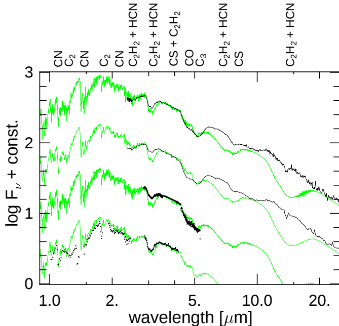
Fig. 9. Comparison of l52t31c14u4pim15 model spectra with observations of V460 Cyg. The model phase is 0.55 in all cases. On top of the figure the main contributing molecules are labelled.
