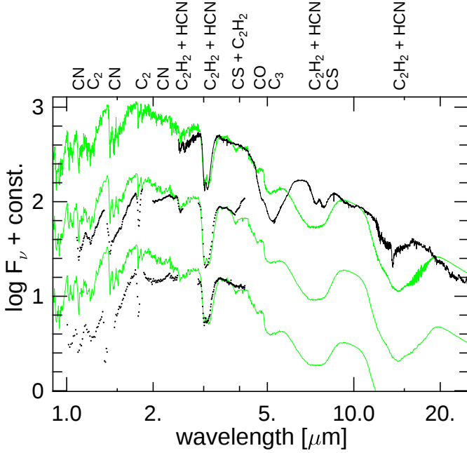
Fig. 11. Comparison of l52t30c20u2pm20 model spectra (grey lines) with the following observational data (black lines) of T Lyr (from top to bottom): one ISO SWS06 spectrum, one spectrum from Joyce, and one spectrum from Lázaro et al. (1994). The model phases are (from top to bottom): 0.61, 0.52, and 0.09. On top of the figure the main contributing molecules are labelled.
