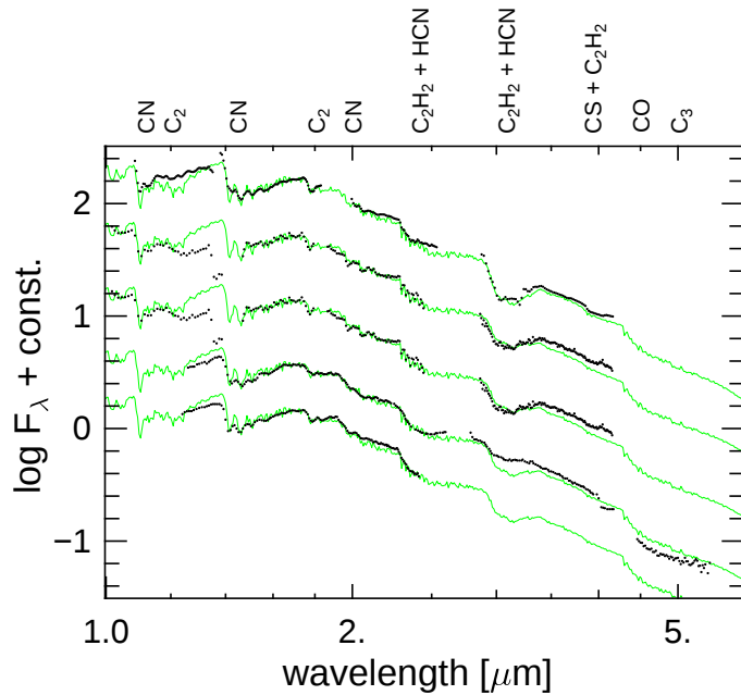
Fig. 3. Comparison of 152t32c11u4 model spectra (grey lines) with the following observational data (black lines) of TX Psc (from top to bottom): one spectrum from Joyce (1998); two spectra from Lázaro et al. (1994); and two KAO spectra. The model phases are (from top to bottom): 0.83, 0.66, 0.71, 0.71, and 0.66. On top of the figure the main contributing molecules are labelled.
