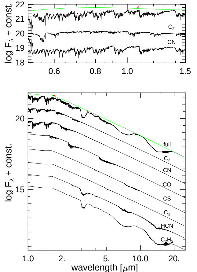
Fig. 1. Upper panel: Full synthetic spectrum at minimum phase of model l52t32c11u4 in the wavelength region between 0.5 and 1.5 \mu\text{m} (top black line), the continuum (grey line) and the contributions of \text{C}_2 , and CN. Lower panel: Full synthetic spectrum in the wavelength region between 1 and 25 \mu\text{m} (black line), the continuum (grey line) and the contributions of \text{C}_2 , CN, CO, CS, \text{C}_3 , HCN, and \text{C}_2\text{H}_2 . Crosses denote wavelengths which were used to normalise observations and model spectra.
