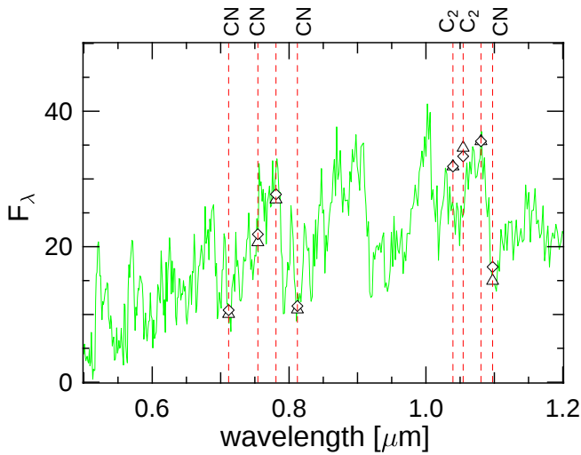
Fig. 7. Comparison of a l52t34c12u2p minimum (phase 0.51) model spectrum with the Baumert observations of V460 Cyg. The maximum values of his colour measurements are denoted by triangles, the minimum values by diamonds. On top of the figure the main contributing molecule is labelled.
