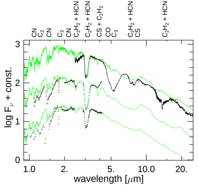
Fig. 12. Comparison of l70t28c16u4 model spectra (grey lines) with observational data (black lines) of T Lyr. The model phases are (from top to bottom): 0.09, 0.82, and 0.00. On top of the figure the main contributing molecules are labelled.
