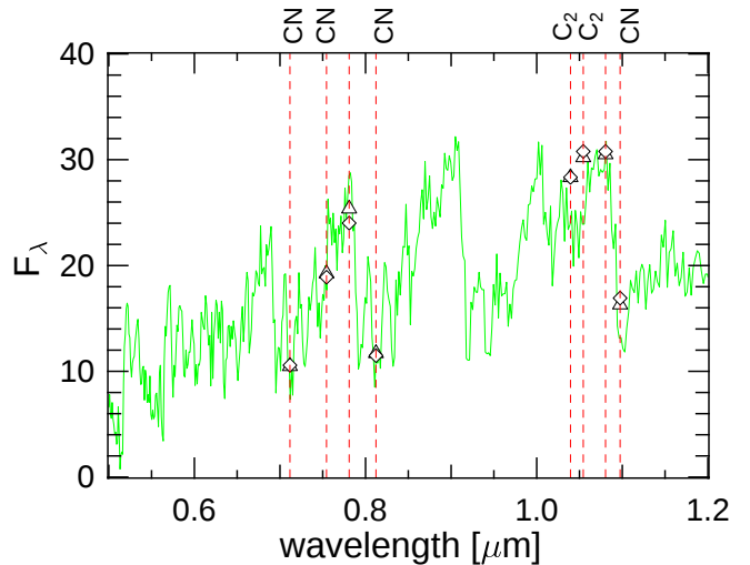
Fig. 2. Comparison of a l52t32c11u4 minimum (phase 0.50) model spectrum with the Baumert observations of TX Psc. The maximum values of his colour measurements are denoted by triangles, the minimum values by diamonds. On top of the figure the main contributing molecule is labelled.
