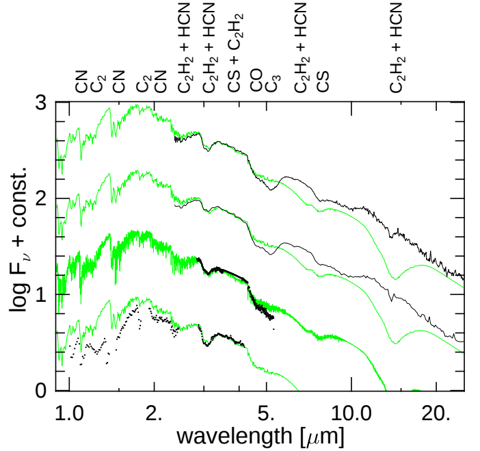
Fig. 8. Comparison of l52t34c12u2p model spectra (grey lines) with the following observational data (black lines) of V460 Cyg (from top to bottom): two ISO SWS01 spectra, one ISO SWS06 spectrum, and one spectrum from Lázaro et al. (1994). The model phases are (from top to bottom): 0.54, 0.56, 0.56, and 0.57. On top of the figure the main contributing molecules are labelled.
