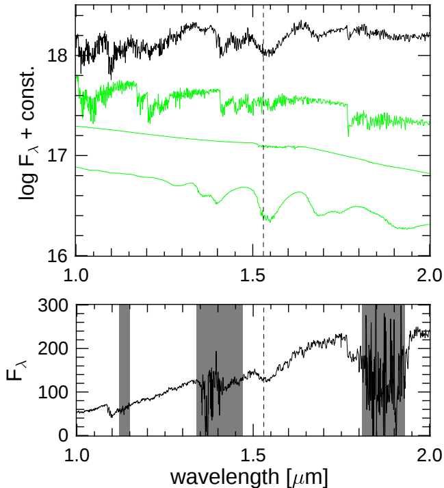
Fig. 14. Full synthetic spectrum at minimum phase of model 170t28c14u5 in the wavelength region between 1 and 2 \mu\text{m} (black line in upper panel) and the contributions of \text{C}_2 , HCN and \text{C}_2\text{H}_2 (grey lines; from top to bottom) to the synthetic spectrum. The dotted line marks the short-wavelength edge of the 1.53 \mu\text{m} feature which is observed in cool carbon-rich Miras (e.g. in R Lep; lower panel). The grey shaded areas mark regions of the spectra which are contaminated by the Earth's atmosphere.
