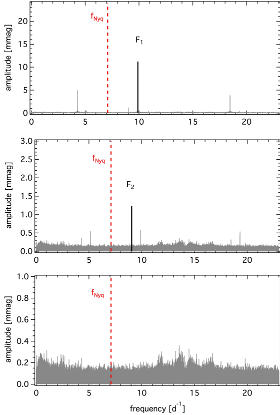
Fig. 4. Amplitude spectra of the SMEI data: Original data with F_1 identified ( top panel ), amplitude spectra after pre-whitening with F_1 and showing F_2 ( middle panel ), and residuals after pre-whitening F_1 and F_2 ( bottom panel ). The position of the Nyquist frequency is marked in red.
