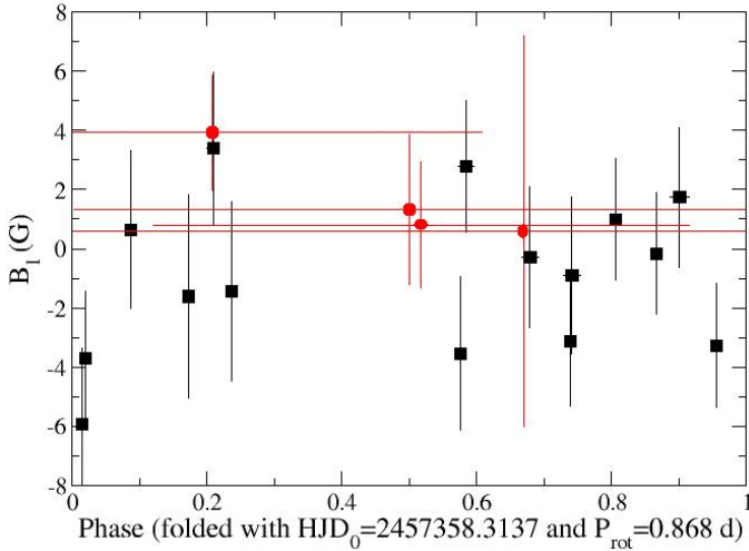
Fig. 11. Longitudinal magnetic field values folded with the rotation period 0.868 d, with phases calculated relative to \text{HJD}_0 = 2457358.3137 corresponding to the start of the 2015 observations. The red symbols indicate the data obtained in 2013 and 2014, which thus have a much larger phase error compared to the 2015 data set.
