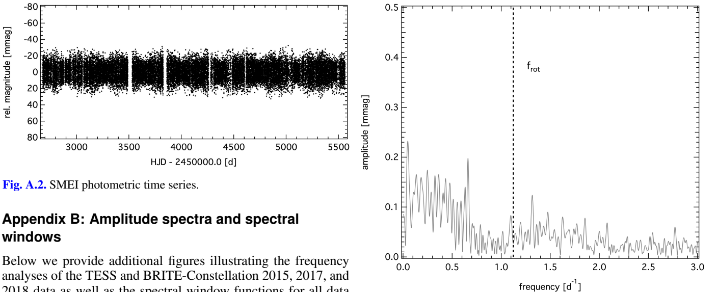
Fig. B.1. Zoom into the low-frequency domain of the amplitude spectrum of the original TESS data before application of a Gaussian filter. The position of the rotation frequency as determined by Che et al. (2011) is indicated with a dashed line.
