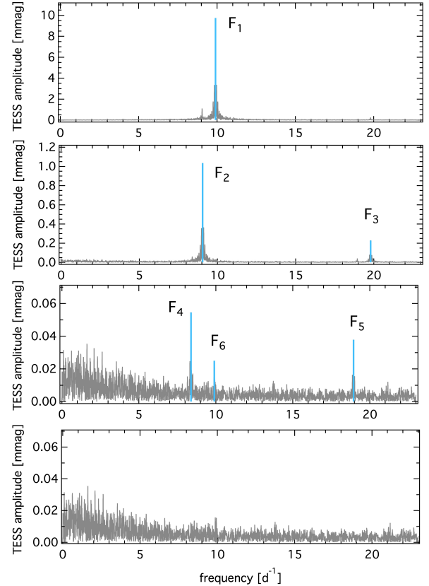
Fig. 5. Fourier analysis of the TESS data: The amplitude spectrum of the original data with F_1 identified ( top panel ), amplitude spectrum after pre-whitening F_1 ( second panel from the top ), amplitude spectrum after pre-whitening F_1 , F_2 , and F_3 ( third panel from the top ), and residual amplitude spectrum after pre-whitening all significant frequencies ( bottom panel ).
