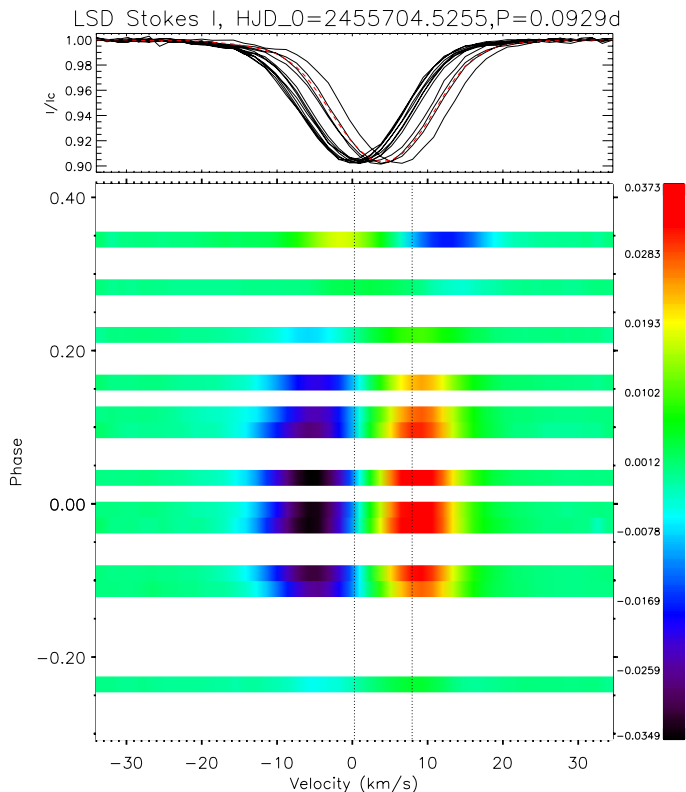
Fig. 6. Top panel: LSD I profiles (black solid lines) of individual subexposures obtained using the mask with all but He lines and the average profile (dashed red line, see text). Bottom: dynamical plot of the residuals of the profiles relative to the mean profile, folded in phase with P = 0.0929 d. The vertical dashed lines indicate \pm 4.112 km s -1 centred on 3.8325 km s -1 and correspond to the excursion domain of the centre of the line.
