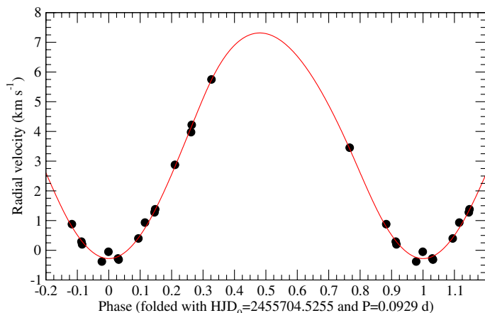
Fig. 5. Radial velocity measurements folded in phase with the period P = 0.0929 d and HJD_0 = 2455704.5255 . The solid red line shows a sinusoidal fit to the data.
