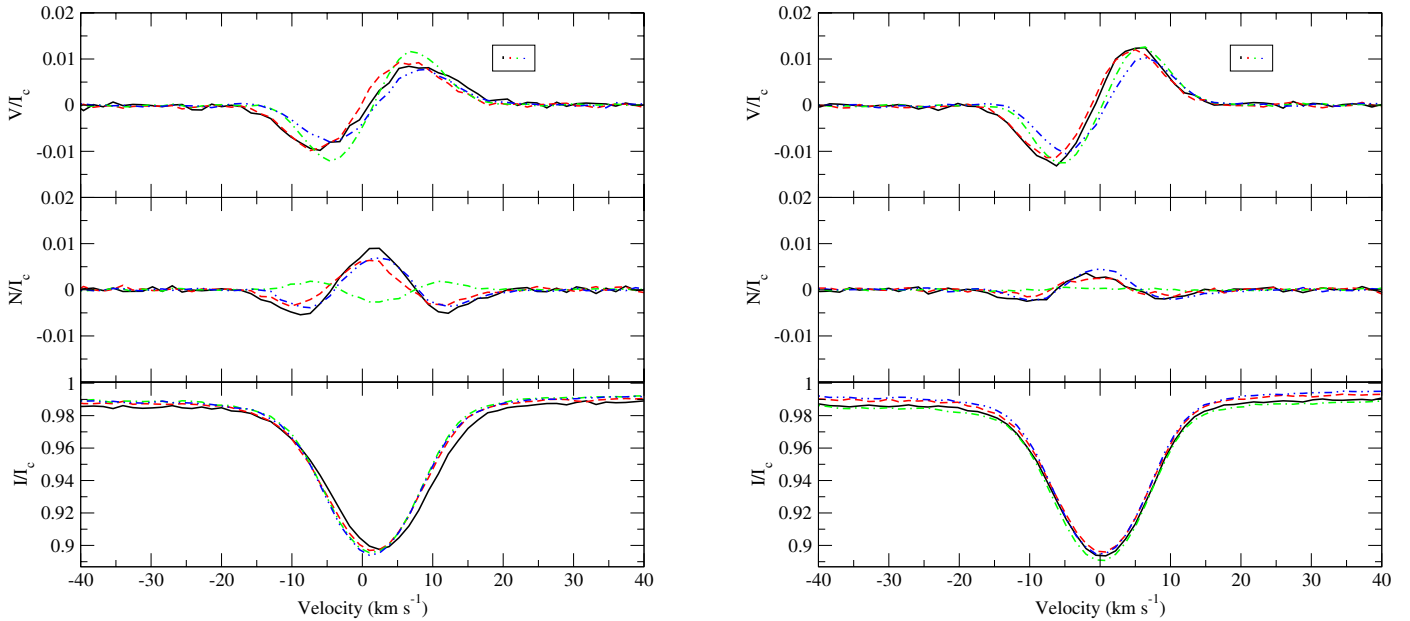
Fig. 8. LSD V (top), N (middle), and I (bottom) profiles of HD 96446 calculated using all photospheric but H and He lines, without (left) or with (right) correction of the radial velocity shifts. Full black line: 23/05, red-dashed line: 24/05 3:30, green dot-dashed line: 24/05 23:14, blue dot-dot-dashed line: 27/05. The mean error bars are plotted in the top box with the respective colour and in chronological order.
