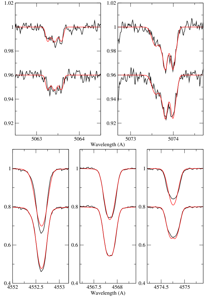
Fig. 9. Upper panel: LTE fit of strongly Zeeman split Fe III lines at 5063 and 5074 Å with \langle |B| \rangle = 4800 \text{ G} and v \sin i = 3 \text{ km s}^{-1} . The fits are shown to the two spectra (#3 and #4) that clearly reveal splitting of the 5074 Å line. Lower panel: comparison of LTE fits to Si III 4552, 4567 and 4574 lines in spectrum #3 with \xi_t = 5 , v \sin i = 6 \text{ km s}^{-1} and no magnetic field (upper curves), to LTE fits (lower curves) with the magnetic model of the upper panel.
