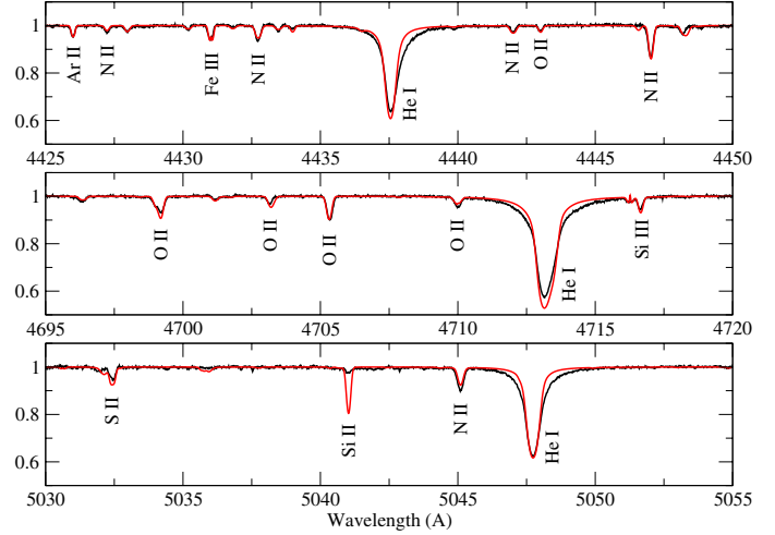
Fig. 10. Three spectral windows in HD 96446, each containing a single He I line. The observed spectrum (#3) is shown in black, the LTE fits in red.
