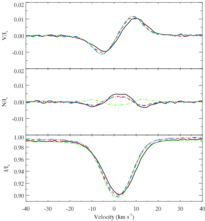
Fig. 7. Simulated Stokes V (top), N (middle) and I (bottom) spectra assuming a -1 kG field and the radial velocity shifts measured in Sect. 4.4.
