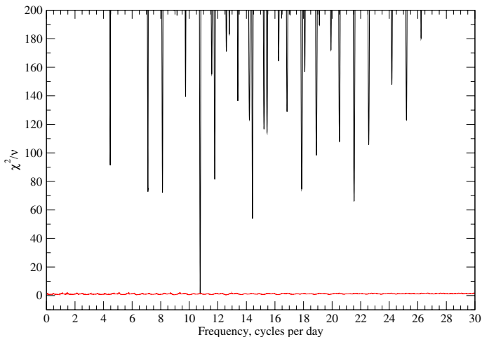
Fig. 4. Frequency spectra of the goodness-of-fit parameter \chi^2/\nu of least squares sine wave fit to our HARPSpol subexposure radial velocity data. The upper fit spectrum shows the fit spectrum to the measured data from Table 3. The lower spectrum is the fit spectrum after a sine wave with period 0.09291 d, amplitude 4.1 km s -1 , and appropriate phase has been subtracted from the measured radial velocities.
