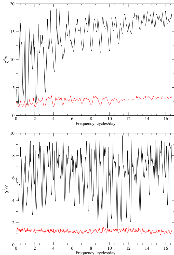
Fig. 1. Frequency spectra of the goodness-of-fit parameter \chi^2/\nu of least squares sine wave fit to 1987 (top) and 1990 (bottom) MB91 V magnitude data. The upper fit spectrum of each panel shows the fit spectrum to the original data. The lower spectrum of the top and bottom panels is the fit spectrum after a sine wave with frequency 1.155 \text{ c d}^{-1} (period 0.866 d), amplitude 11.7 mmag, and with frequency 10.80 \text{ c d}^{-1} (period 0.0926 d), amplitude 9.2 mmag respectively, and appropriate phase, has been subtracted from the measured V magnitudes.
