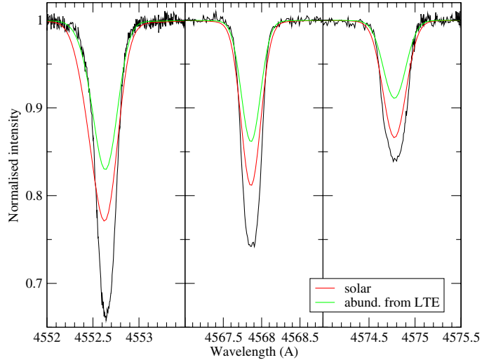
Fig. 12. NLTE models with solar (red line) and LTE abundances (green line) of the Si III triplet.
