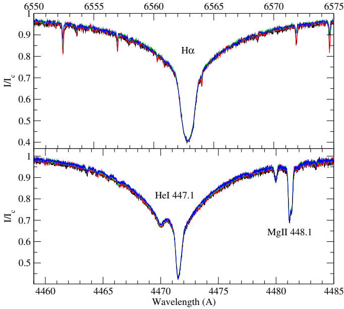
Fig. 2. H\alpha (top panel) and He I 4471 and Mg II 4481 (bottom panel) lines observed in the 4 HARPSPol spectra, superimposed on each other. No variability is observed, in particular no possible emission variability.
