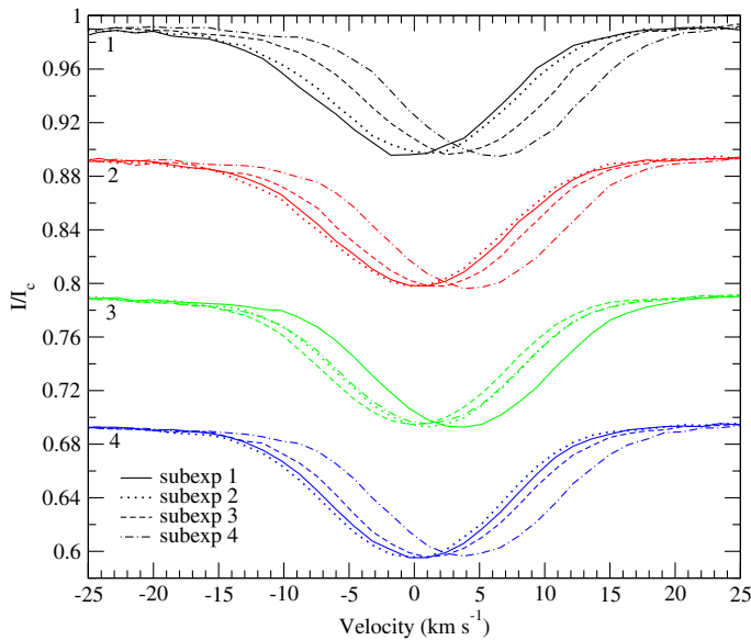
Fig. 3. LSD I profiles of individual subexposures obtained using the mask with all but He lines. The subexposures of the 4 polarisation measurements are shown from top to bottom. The profiles have been arbitrarily shifted by -0.1 , -0.2 and -0.3 in intensity to ease the reading of the figure. The 4 subexposures of each polarisation measurements are drawn with solid, dotted, dashed, and dashed-dotted lines in chronological order.
