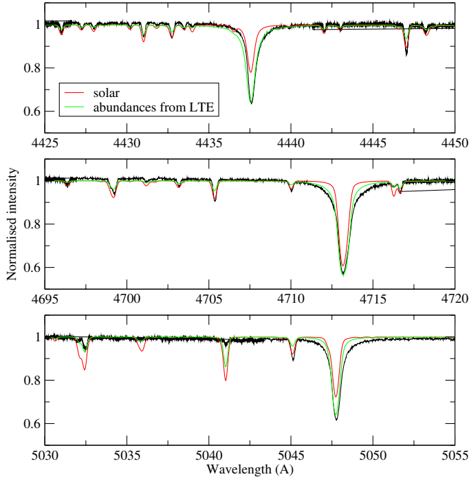
Fig. 11. Same as Fig. 10 but for NLTE models with solar (red line) and LTE abundances (green line).
