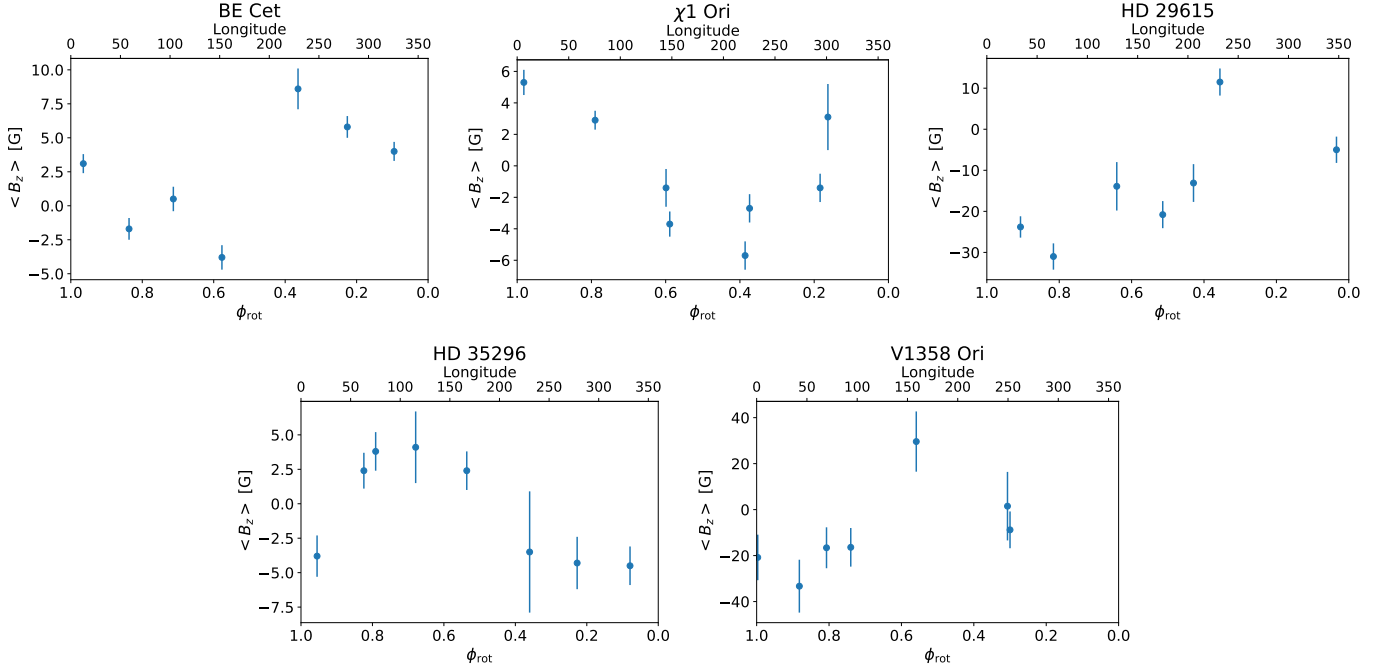
Fig. 1. Mean line-of-sight magnetic field, \langle B_z \rangle , of the observed stars as a function of their rotational phase. The corresponding longitudes on the stellar surface (which is turned towards the observer at that phase) are shown on the top axis. The phases are inverted in order for the longitudes to match those used in the ZDI maps (Figs. 2–6), where the direction of the rotation is chosen to be similar to the Earth’s rotation.
