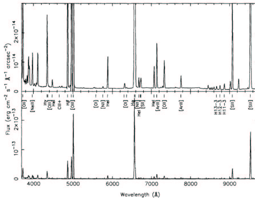
Optical spectrum of the Orion nebula (Baldwin et al. 1991)
